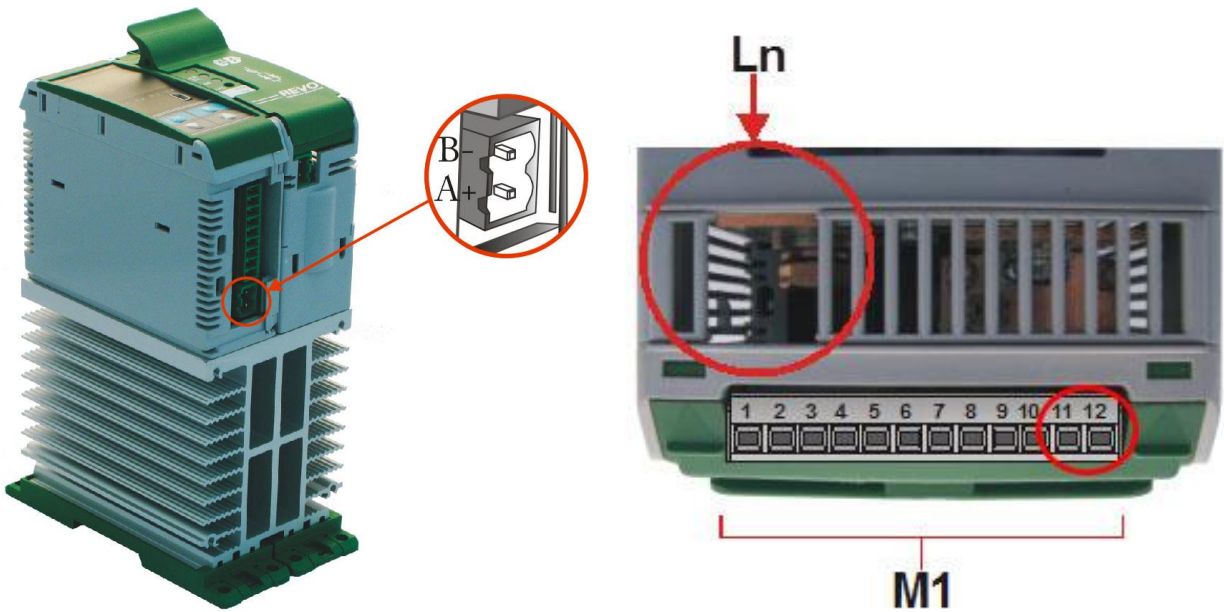
TOP VIEW
